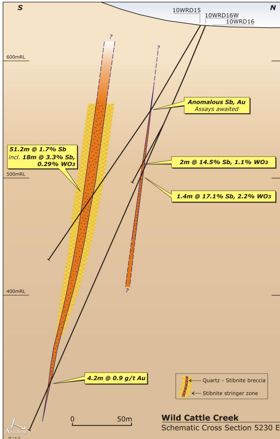
Figure 2 WCC – High grade antimony-tungsten zone (Holes 10WRD16 and 16W)
