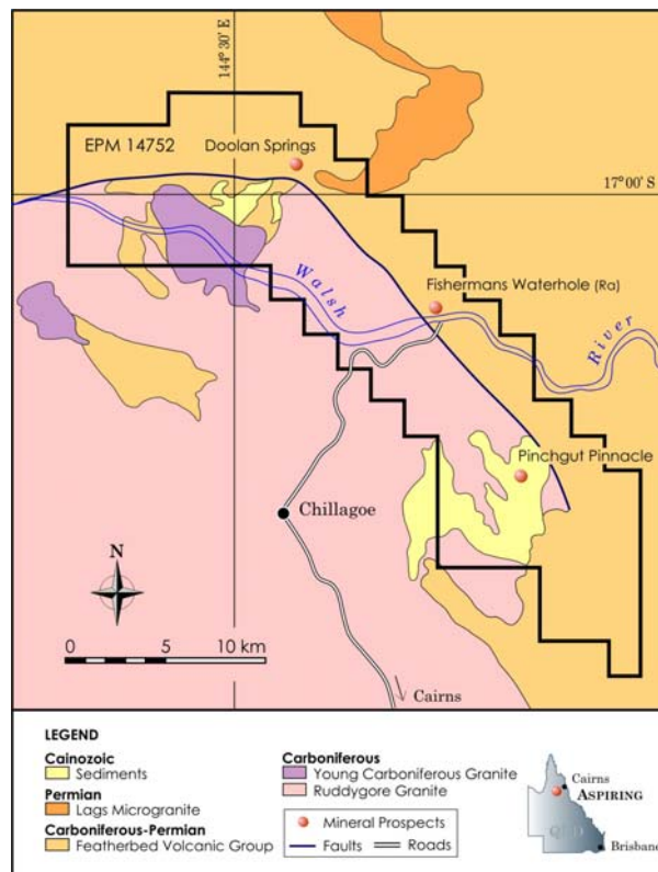
Figure 1 Aspiring Uranium Project Location and Geology Map
